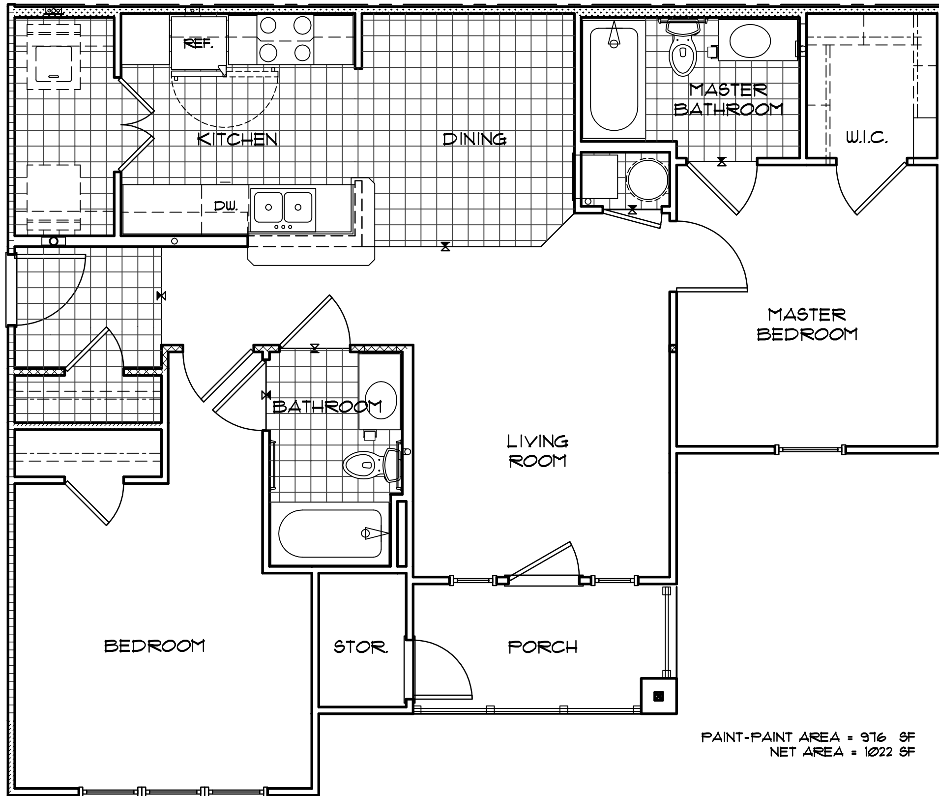
1 2 BEDROOM/2 BATH UNIT 1/4" = 1'-0"
